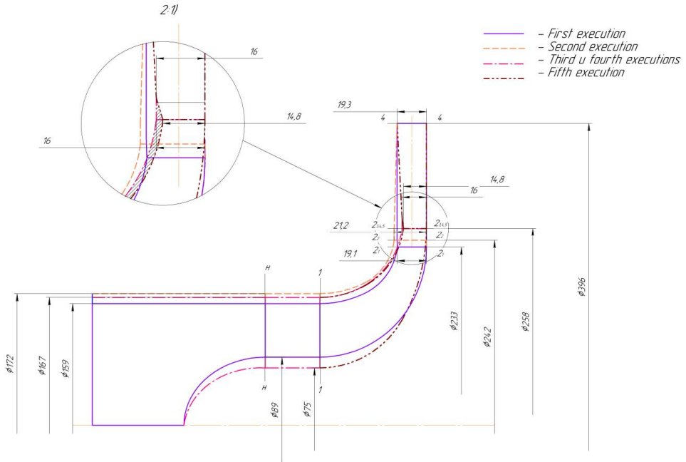
Fig. 1. The centrifugal compressor stage meridional section with control sections and changes in the flow path geometry, depending on optimization approaches (dimensions in mm) in five executions.
