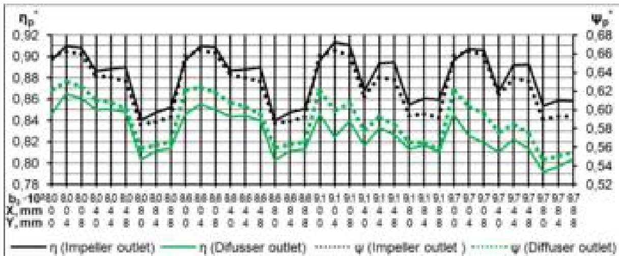
Fig. 7. The results of the optimization of the impeller shroud counter and the width of vane diffuser (b3) with controlled values X and Y.
